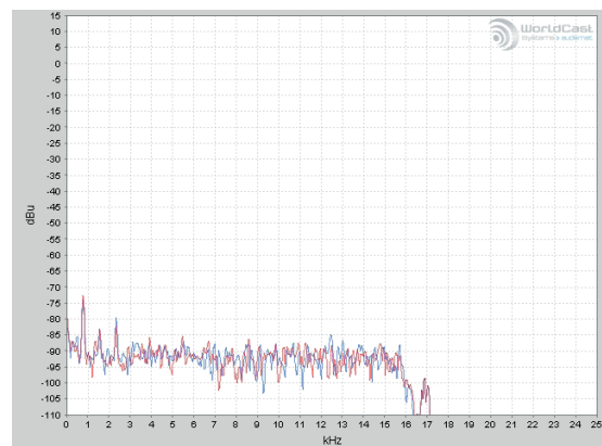
Audemat RDS Encoder audio spectrum
