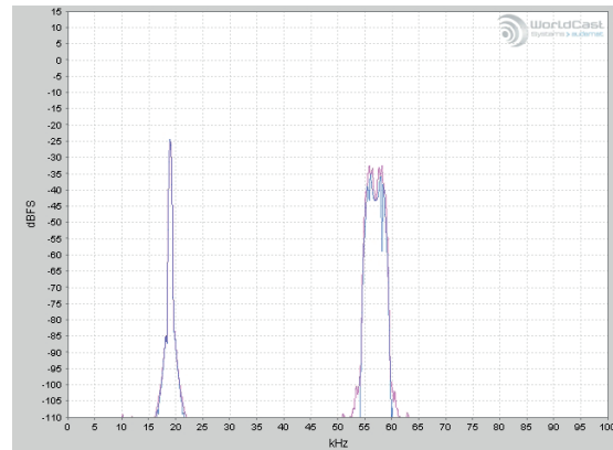
Audemat RDS Encoder MPX Spectrum
