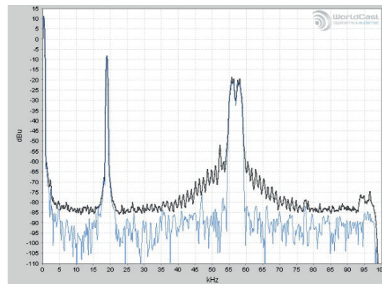
Competitor encoder MXP spectrum
