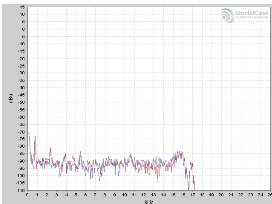
Audemat FMB80 audio spectrum
