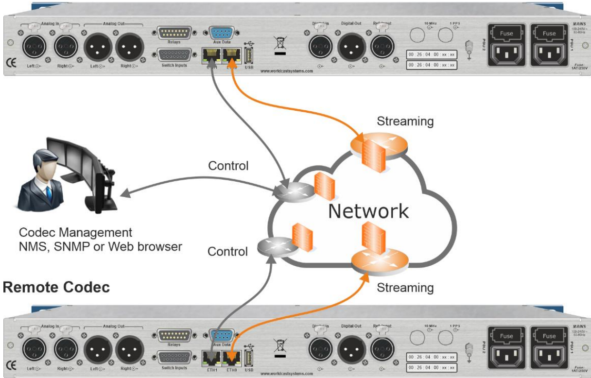
Figure 11: Shows the principle of the Codec installation in a generic network (standard APT IP Codec depicted)
