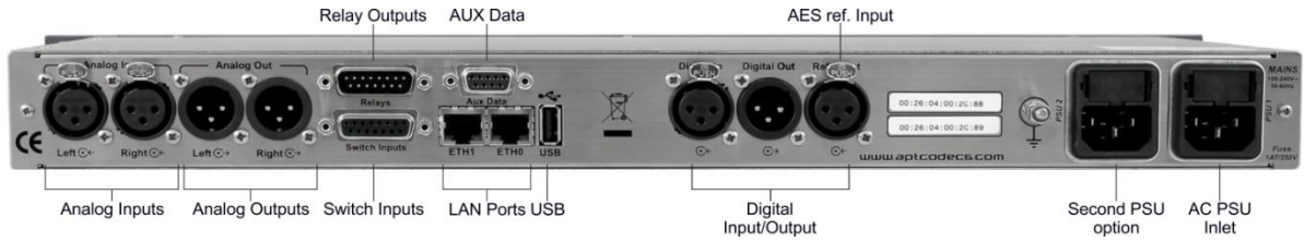
Figure 9: Shows all rear panel components of the standard IP Codec
